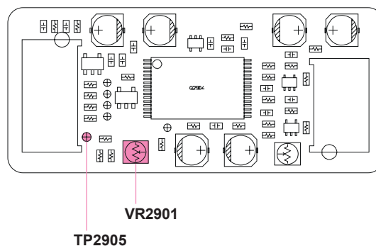
DVS UNIT ALIGNMENT POINTS
