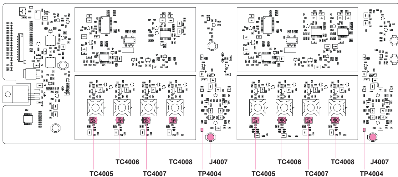
PA-A UNIT ALIGNMENT POINTS
