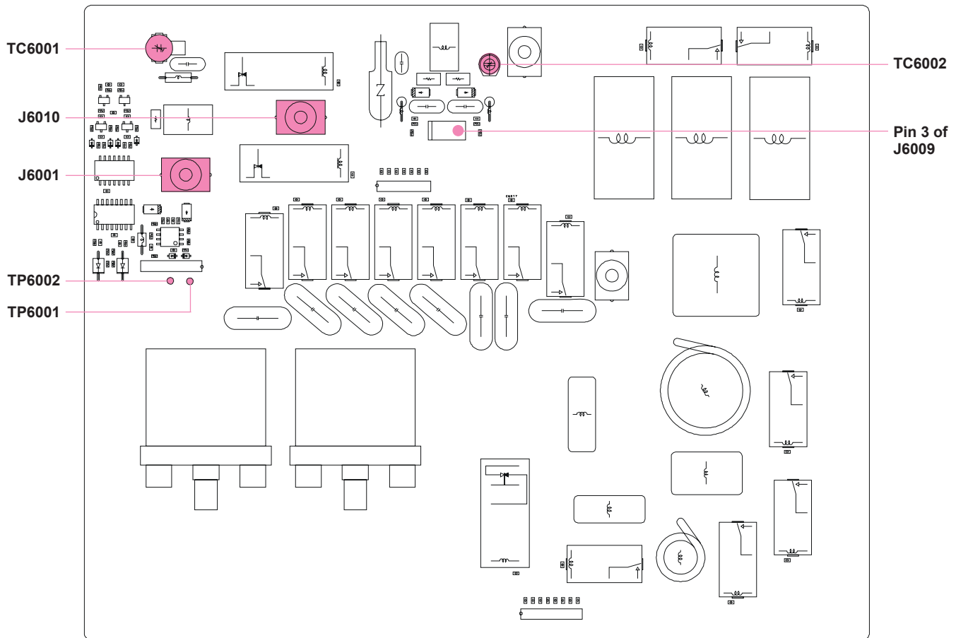
TUNER-MAIN UNIT ALIGNMENT POINTS
