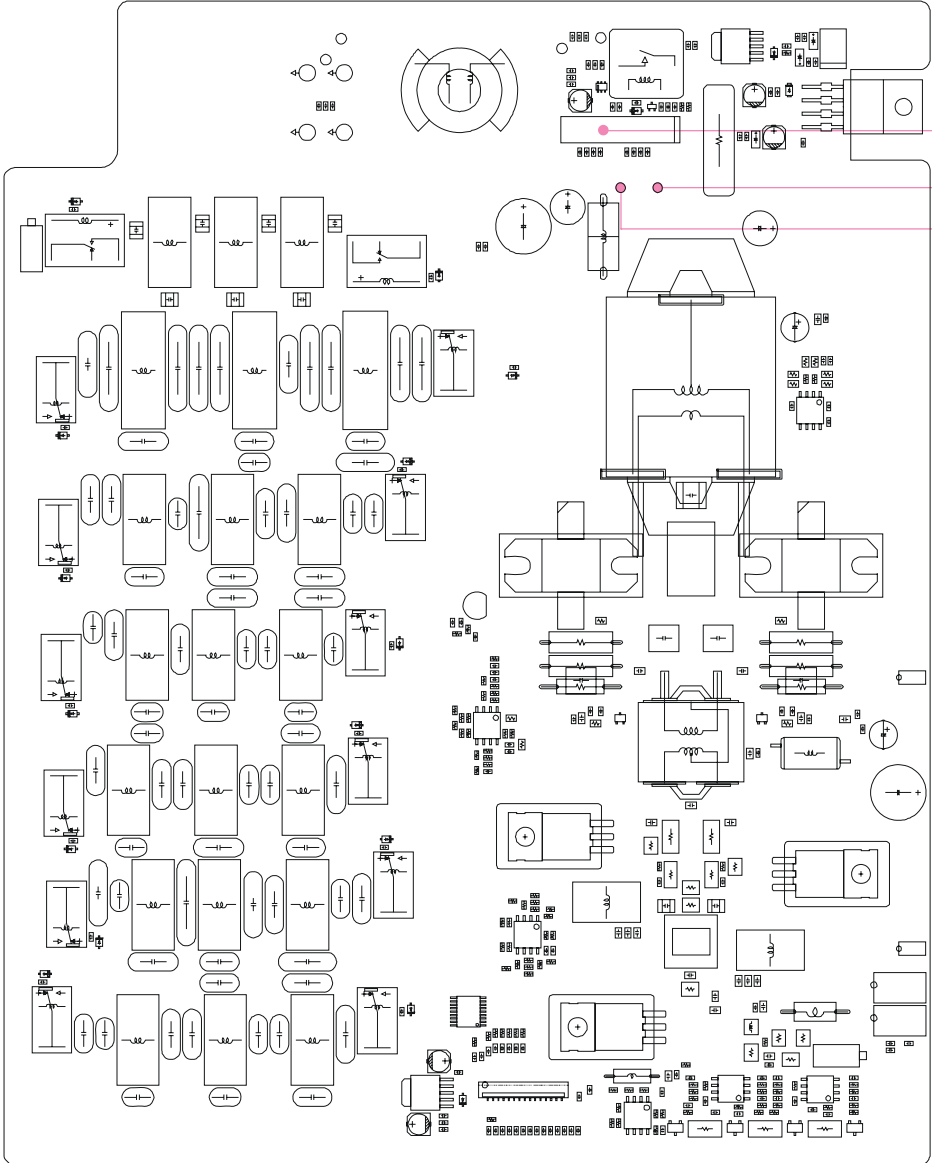
PA-A UNIT ALIGNMENT POINTS
